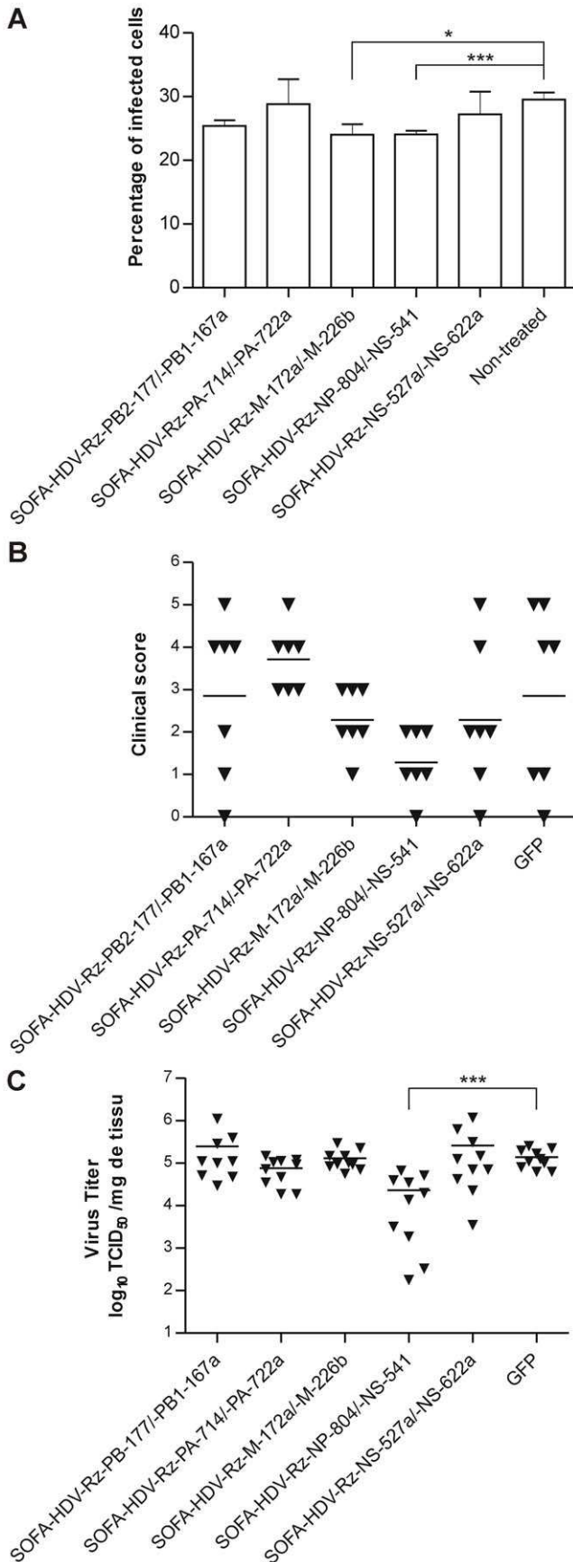
Figure 4. Antiviral activity of SOFA-HDV-Rz (A) in cells and (B and C) in vivo. (A) MDCK cells were transfected with the indicated SOFA-HDV-Rz combinations, and infected with PR8 at a MOI of 0.01 after 24 h. Ten hours later, the cells were fixed and stained with a monoclonal antibody against HA. The percentage of HA-positive cells detected in three independent experiments is shown. Error bars indicate standard deviation. (B and C) BALB/c mice were transfected intranasally with the indicated SOFA-HDV-Rz combinations and challenged with 10 5 50% tissue culture infectious doses (TCID 50 ) of PR8 6 h later. (B) Clinical score on day 3 after infection. The clinical score represents a combination of posture, activity, and weight loss scores evaluated on a 0-1-2 scale as detailed in materials and methods. Results from 2 independent experiments are shown, and each symbol represents one animal. (C) Viral lung titers on day 1 after infection. Animals were sacrificed 24 h after infection and the lung was harvested. Titers are expressed as TCID 50 per g of tissue. Student's t-test: asterisk, P<0.05; three asterisks, P<0.001. doi:10.1371/journal.pone.0027327.g004
