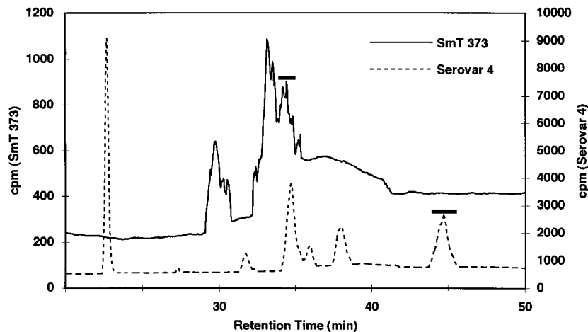
FIG. 1. HPLC distribution of radioactivity in deacylated lipid from M. avium SmT 373 and serovar 4, radiolabeled with [ ^{14} C]phenylalanine. Samples were separated in a mobile phase of 100% chloroform for 10 min and then a 40-min gradient of 0 to 10% methanol in chloroform at a flow rate of 1.0 ml/min; radioactivity was detected by a solid-cell detector (20). Bars, fractions associated with GPL components.
