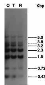
FIG. 2. IS1245 RFLP patterns of M. avium 373 SmO (O), SmT (T), and Rg (R) colony morphotypes. Genomic DNA was digested with the Sal I restriction enzyme and hybridized with IS1245 , nonradioactively labeled by using the Genius system. Sizes of bands were determined from known standards.
