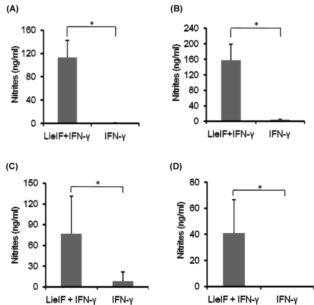
Figure 4. Nitric oxide production (ng/ml) by J774A.1 macrophages upon treatment with LieIF/IFN- \gamma at late (A, B) and early (C, D) time points after L. donovani infection. J774A.1 cells were treated pre-infection (A, C) and post-infection (B, D) with recombinant LieIF (10 \mu g/ml) and recombinant IFN- \gamma (1 ng/ml). Nitrite accumulation in the medium was measured by addition of Griess reagent, absorbance reading of the reaction product at 570 nm. All data are presented as the mean \pm S.D of at least three independent experiments. Asterisks indicate statistically significant production of NO ( p \leq 0.05 ). doi:10.1371/journal.pone.0097319.g004
