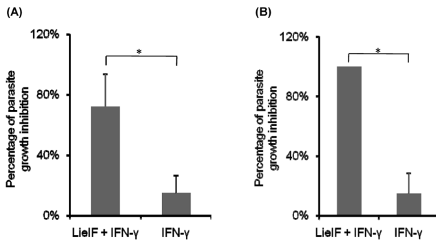
Figure 3. Effect of post-infection treatment of J774A.1 macrophages with LieIF/IFN- \gamma in intracellular L. donovani growth inhibition. (A) at early (19 h) and (B) late (72 h) time points after infection. J774A.1 cells were stimulated with 10 \mu g/ml recombinant LieIF and 1 ng/ml recombinant IFN- \gamma . L. donovani growth inhibition was determined by the colorimetric method alamarBlue and OD was measured at 570/630 nm. Data are presented as the mean \pm S.D of at least three independent experiments. Asterisks indicate statistically significant inhibition of parasite growth ( p \leq 0.05 ). doi:10.1371/journal.pone.0097319.g003
