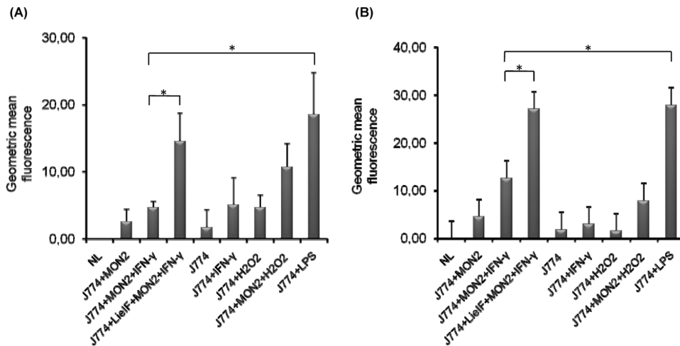
Figure 5. ROS generation by J774A.1 macrophages pre- and post- infection treated (A and B, respectively) with recombinant LieIF (10 \mu g/ml) and recombinant IFN- \gamma (1 ng/ml). ROS generation was determined at the late time point (72 h) after L. donovani infection. Cells were labelled with 5 \mu M H 2 DCFDA fluorescent probe and fluorescence of cells reacting with the probe was estimated by FACS analysis. All data are presented as the mean \pm S.D of at least three independent experiments. Asterisks indicate statistically significant production of ROS ( p \leq 0.05 ) compared to the control group of infected J774A.1 cells stimulated with IFN- \gamma (J774 + MON2 + IFN- \gamma ). NL: for medium only; MON2: for the MHOM/IN/1996/THAK35 L. donovani strain used. doi:10.1371/journal.pone.0097319.g005
