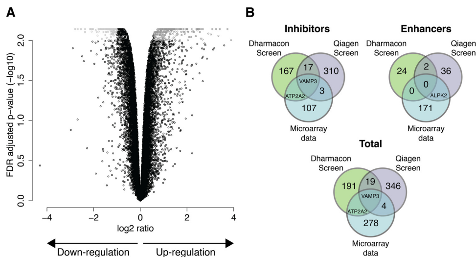
FIG 4 miR-142-3p regulates VAMP3. (A) Microarray chips were used to define the genes regulated by miR-142-3p. The x axis of the volcano plot indicates the magnitude of gene expression changes, on a \log_2 scale, and the y axis shows the corrected P value for multiple comparisons. The correction was performed using the false-discovery rate (FDR) method, and values were log transformed and multiplied by -1 . Data represent the combination of four independent experiments. (B) Overlaps of potential hits between microarray data obtained for miR-142-3p and both siRNA screens.
