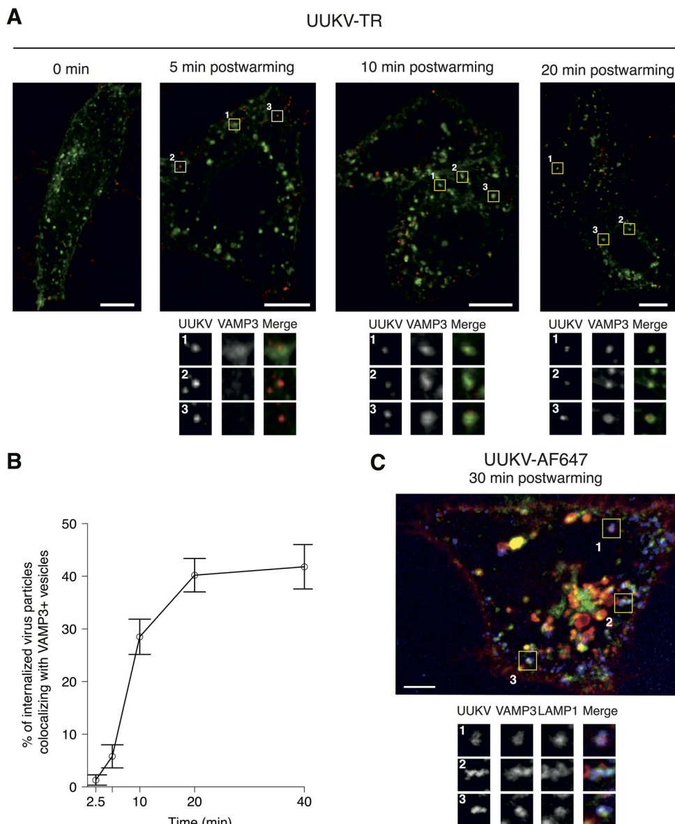
FIG 6 UUKV associates with VAMP3 and LAMP1. (A) Bodipy Texas Red-conjugated UUKV (UUKV-TR; MOI, ~10) was bound to EGFP-VAMP3-expressing cells on ice. Cells were washed, rapidly warmed for up to 40 min, and fixed. UUKV (red) and EGFP-VAMP3 (green) were imaged in one focal plane by confocal microscopy. Magnifications of the association between UUKV and green vesicles (yellow squares) or noncolocalizing, internalized particles (white squares) are shown on the bottom. Bars, 10 \mu m. (B) The percentage of viruses colocalizing with the marker EGFP-VAMP3 at different times postwarming was calculated from series of z stacks, as described for those shown in panel A, and merged to one plane. Cells ( n = 10 ) were counted in 10 independent fields for each time point. Error bars indicate the standard error (SE) of the means of the counted cells. The data are representative of three independent experiments. (C) Entry of prebound AF647-labeled UUKV (UUKV-AF647; MOI, ~10) into cells expressing EGFP-VAMP3 and RFP-LAMP1, based on confocal microscopy. Viruses were internalized at 37°C for 30 min. One focal plane is shown; UUKV is seen in blue, cell vesicles containing EGFP-VAMP3 are green, and RFP-LAMP1 is red. Magnifications of association between VAMP3 + LAMP1 + vesicles and internalized UUKV are shown on the bottom (yellow squares). Bar, 5 \mu m.
